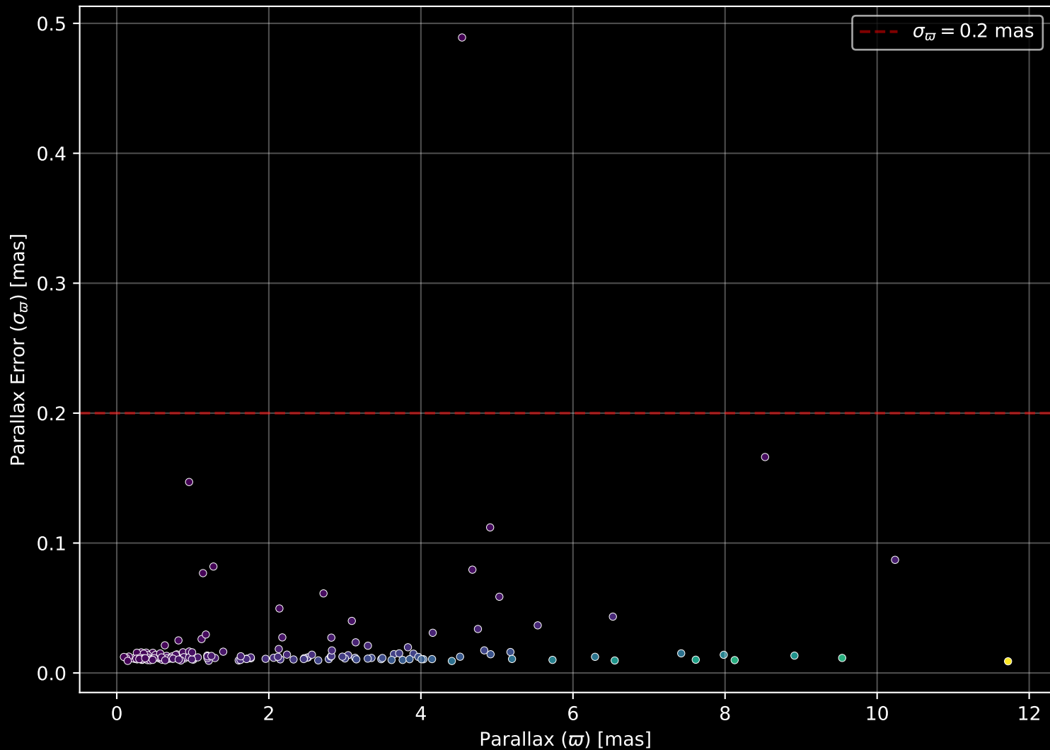
APOGEE DR17 Field: [277-24-O_TESS] Parallax Quality (n= 150)
