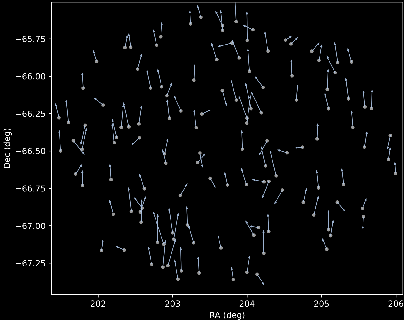
APOGEE DR17 Cluster 1 Proper Motion Vectors (n=125)
