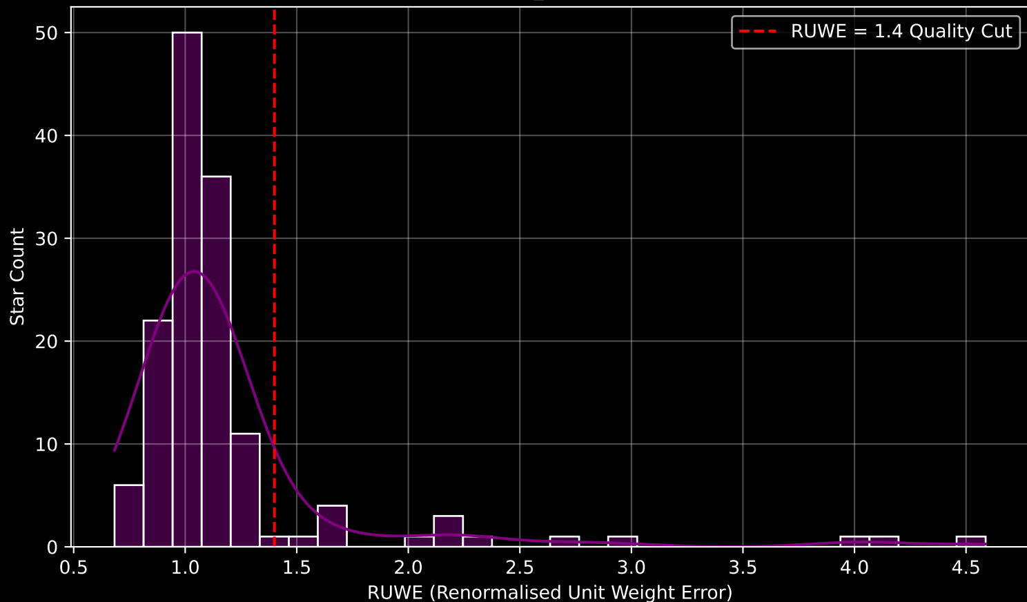
GAPOGEE DR17 Field [277-24-O_TESS] RUWE Distribution (n= 141)
