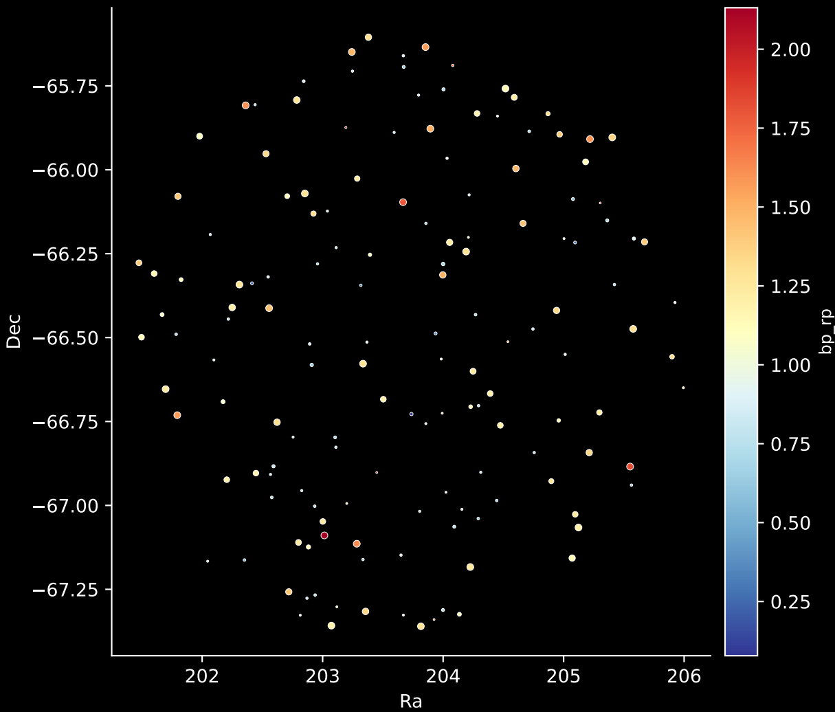
APOGEE DR17 Field: [277-24-O_TESS] Stars: 150
