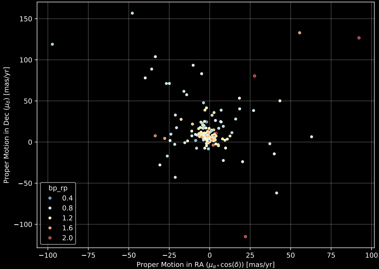
APOGEE DR17 Field: [277-24-O_TESS] Proper Motion Diagram (n= 150)
