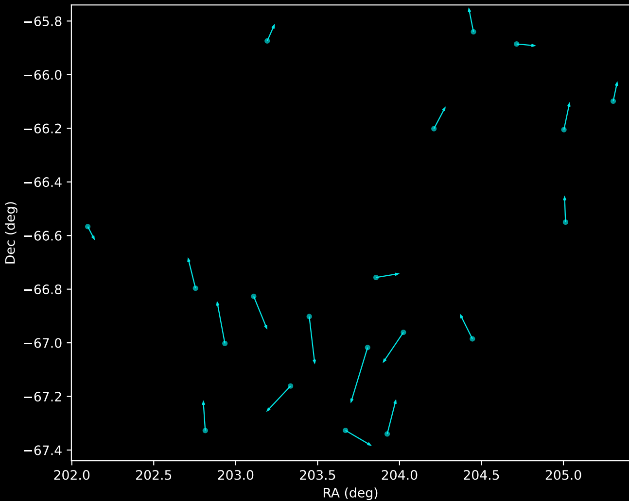
APOGEE DR17 Noise Stream Proper Motion Vectors (n=20)
