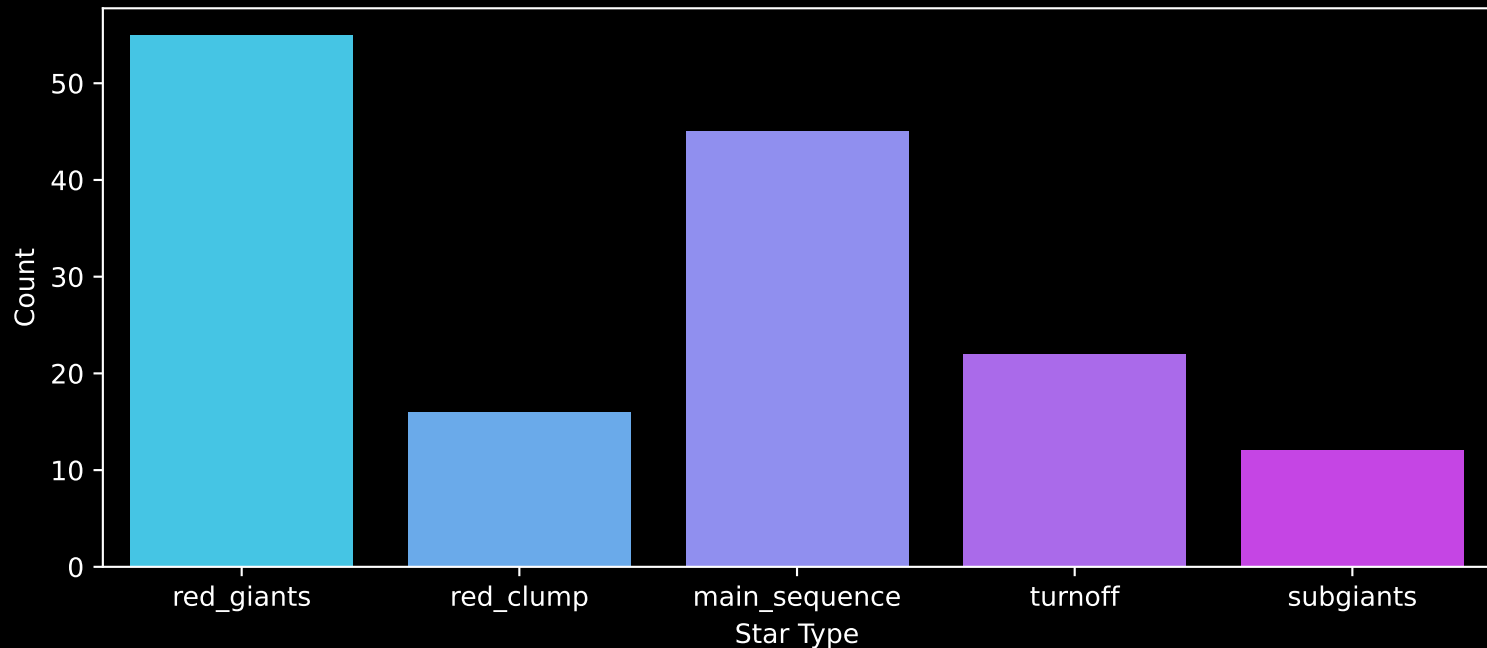
APOGEE DR17 Field: [277-24-O_TESS] Count plot of Star Type
