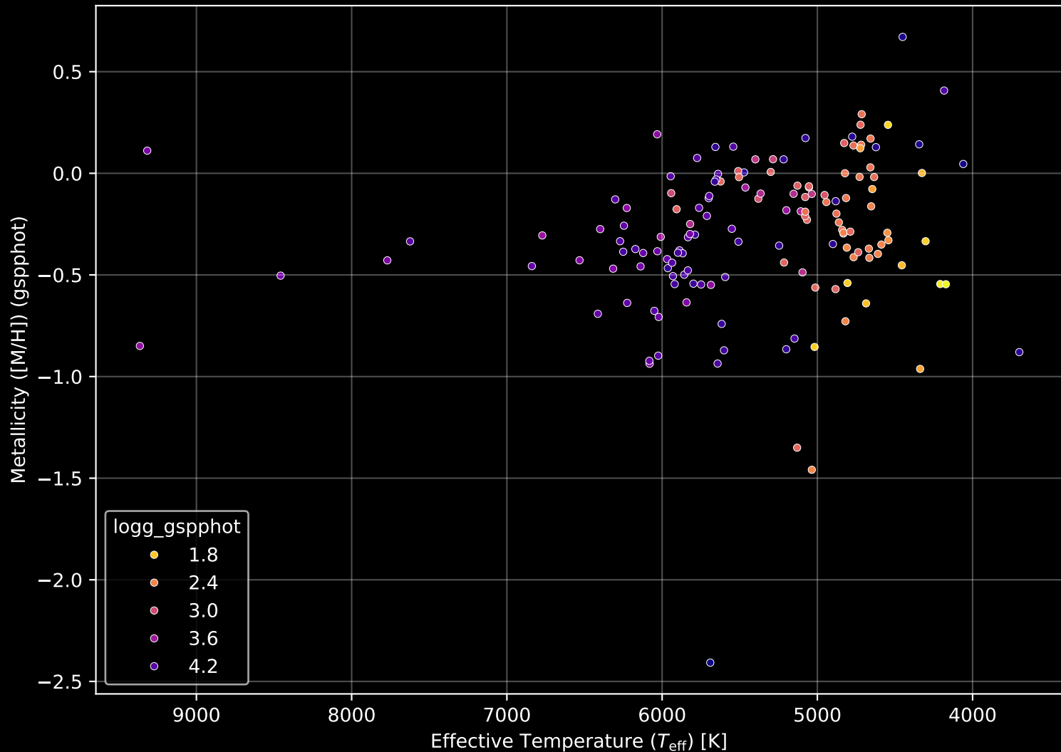
APOGEE DR17 Field: [277-24-O_TESS] Stellar Population Parameters (n= 150)
