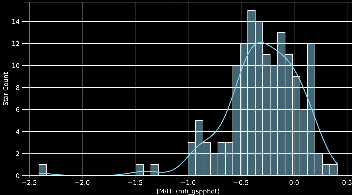
APOGEE DR17 Field: [277-24-O_TESS [M/H] (mh_gspphot) (n= 149)
